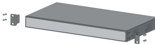
Figure 3-1 Fix bracket
